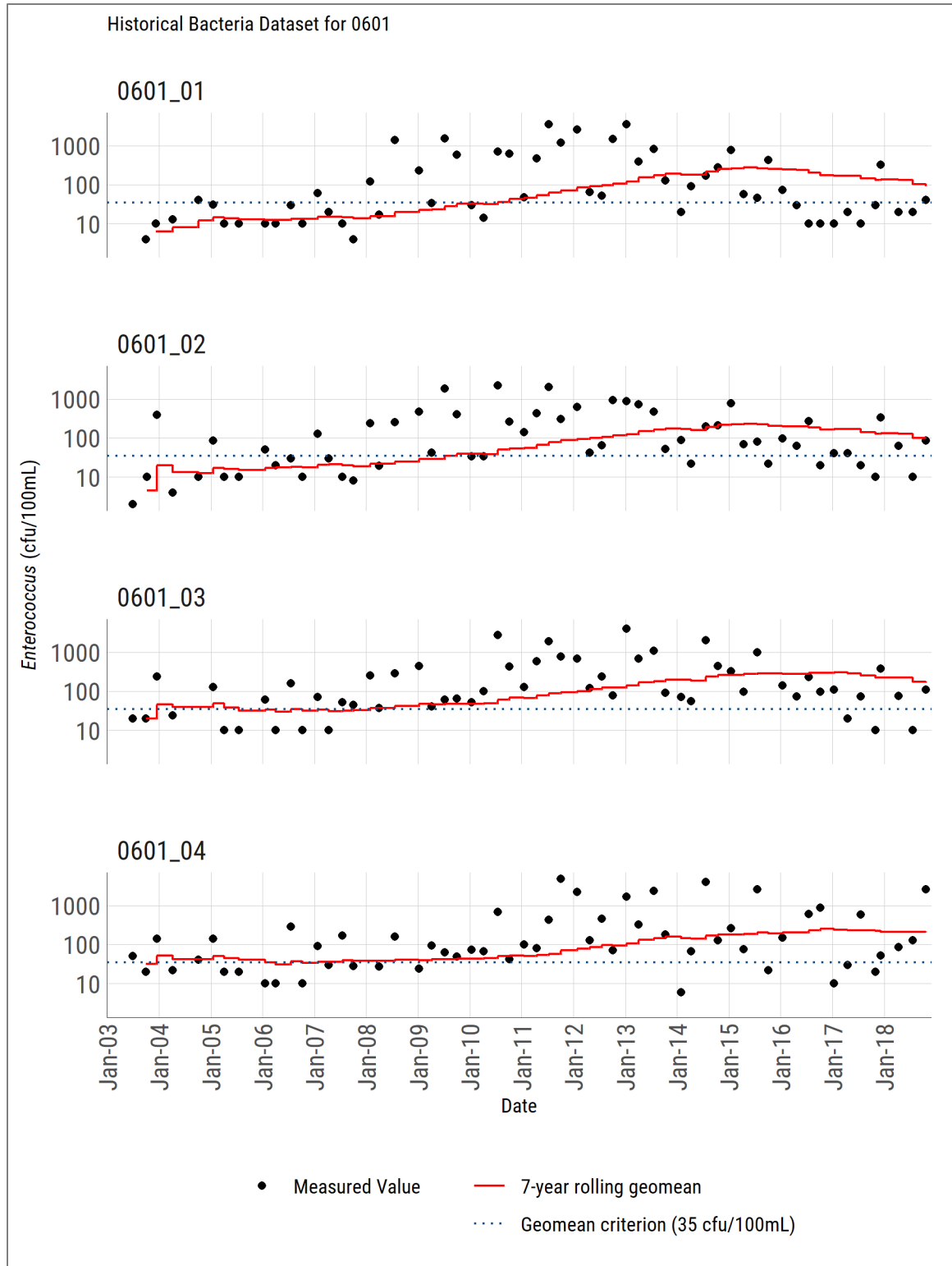
Figure 11. Summary plots of historical bacteria datasets for impaired AUs in Neches River Tidal (0601) including the 7-year rolling geometric mean from June 2003 through December 2018.
