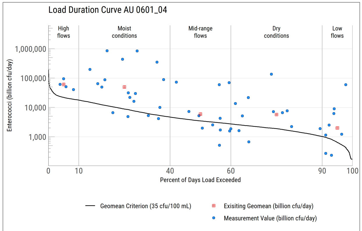
Figure 30. Load duration curve for Neches River Tidal (0601_04) at SWQM station 10575.
