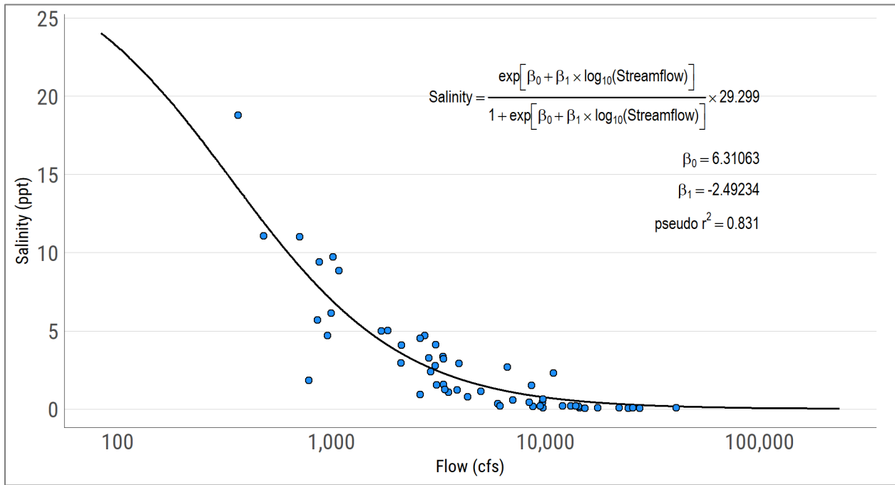
Figure 20. Salinity to flow regression for SWQM station 10570.
