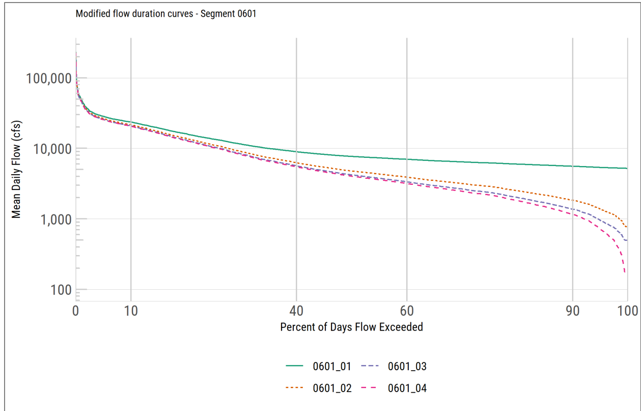
Figure 29. Modified flow duration curves for Neches River Tidal.
