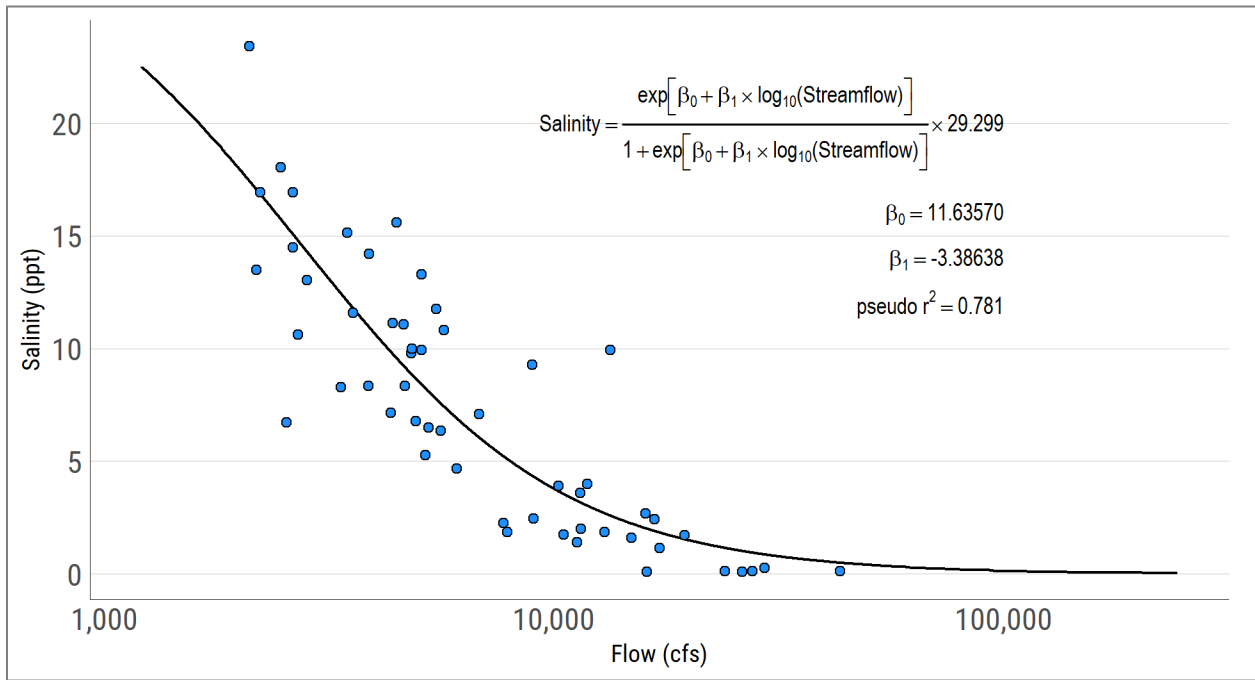
Figure 22. Salinity to flow regression for SWQM station 10563.
