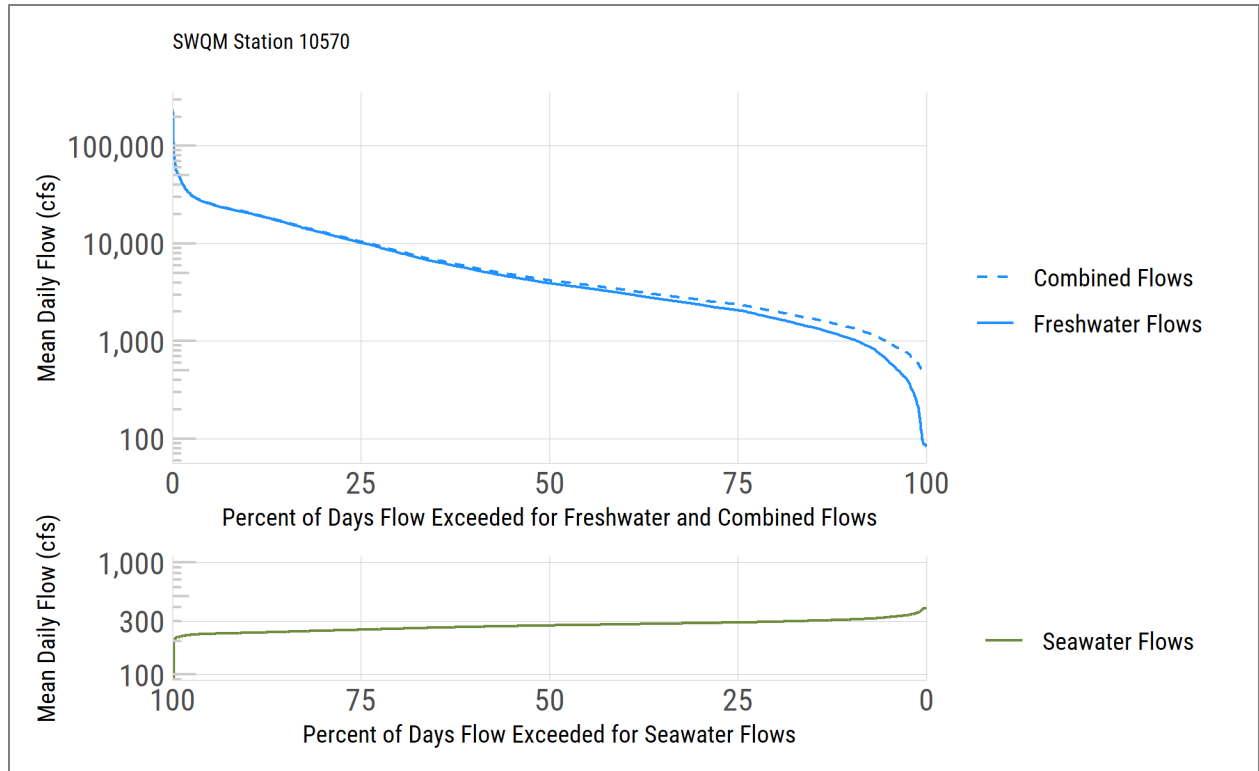
Figure 26. Flow duration curve components for SWQM Station 10570 (0601_03).
