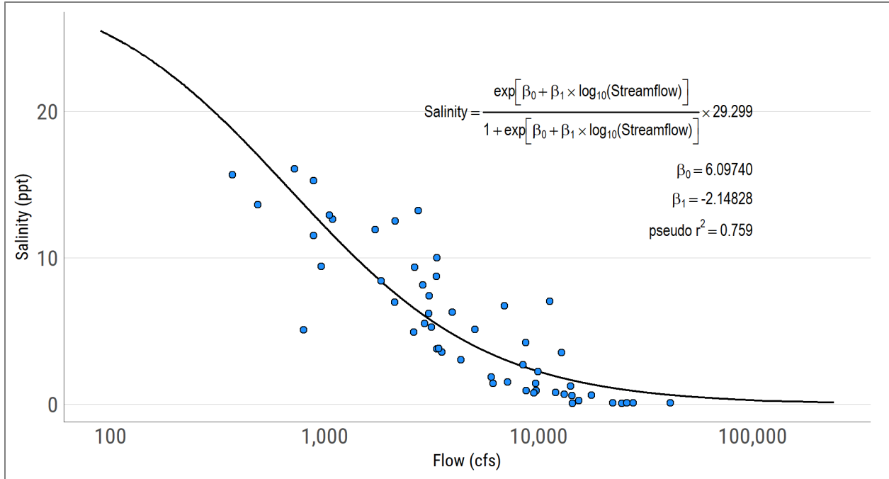
Figure 21. Salinity to flow regression for SWQM station 10566.
