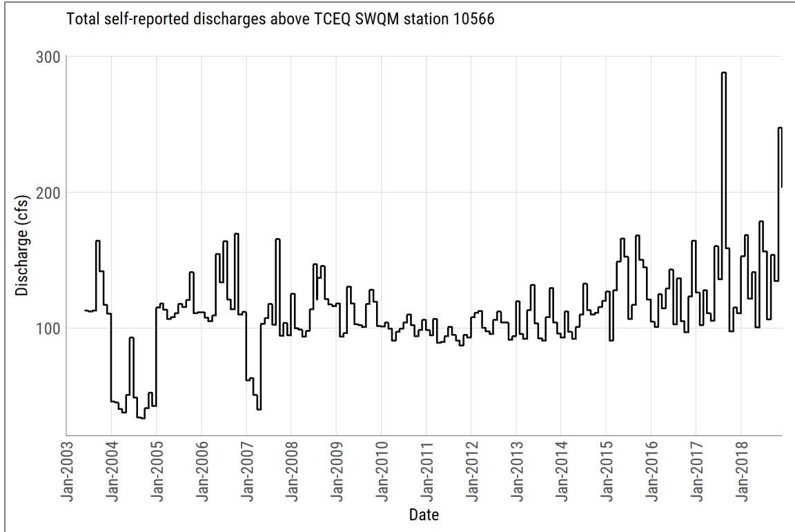
Figure 17. Reported discharge volumes for permitted facilities upstream of SWQM station 10566.
