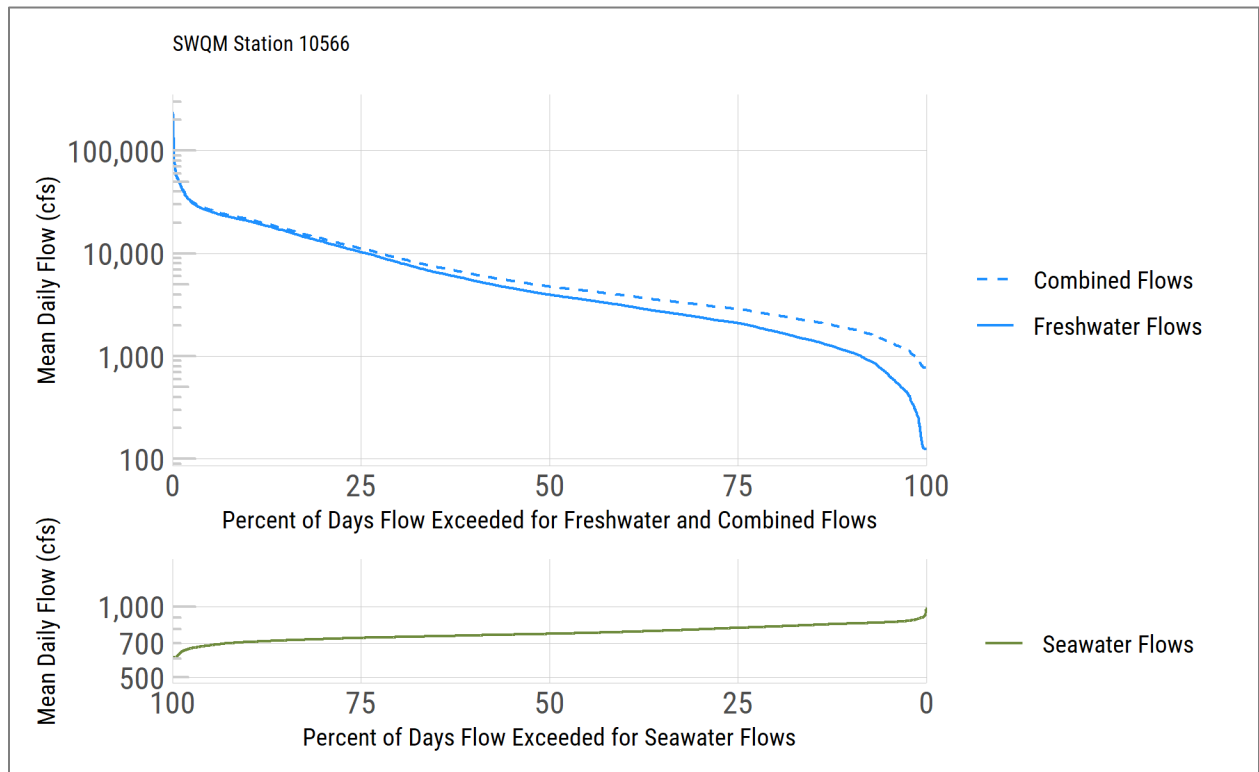
Figure 27. Flow duration curve components for SWQM Station 10566 (0601_02).
