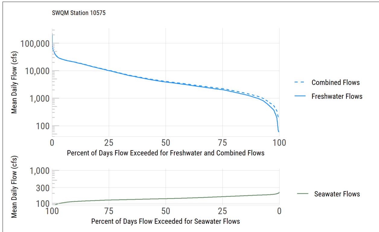
Figure 25. Flow duration curve components for SWQM Station 10575 (0601_04).
