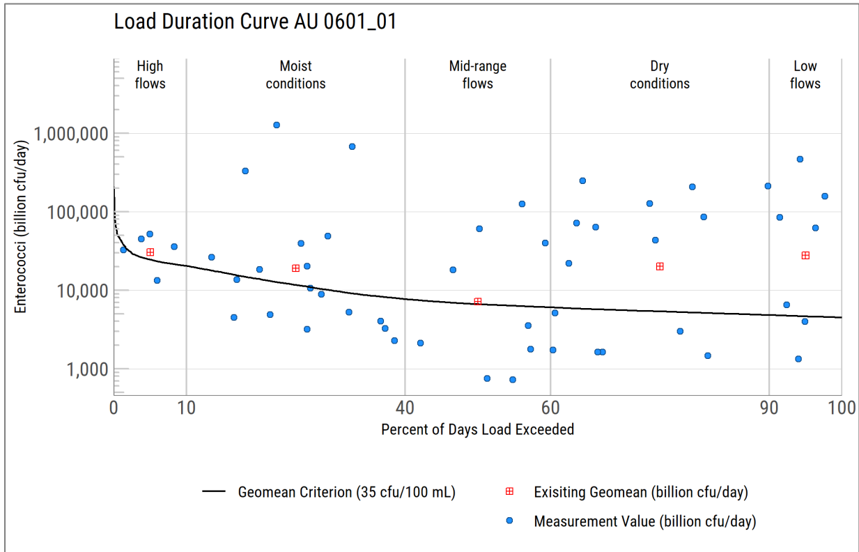
Figure 33. Load duration curve for Neches River Tidal (0601_01) at SWQM station 10563.
