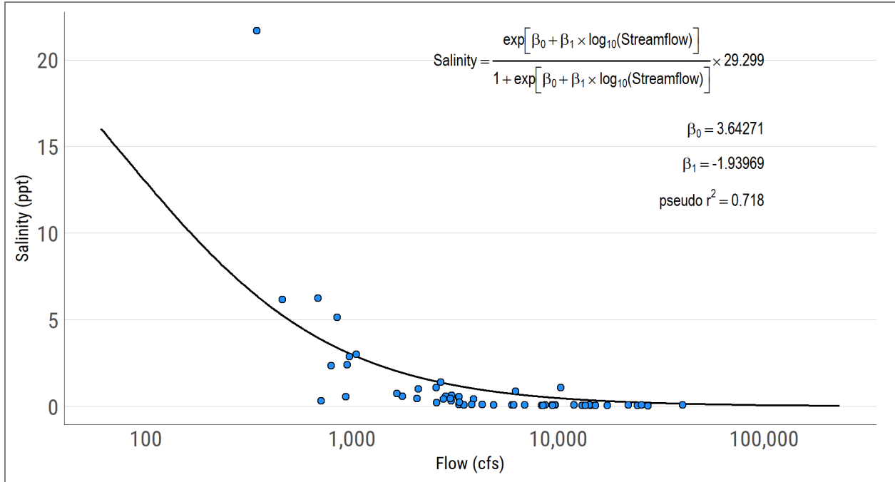
Figure 19. Salinity to flow regression for SWQM station 10575.
