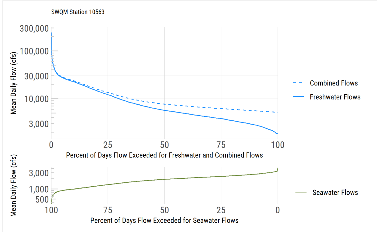
Figure 28. Flow duration curve components for SWQM Station 10563 (0601_01).
