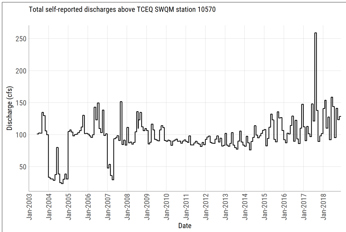
Figure 16. Reported discharge volumes for permitted facilities upstream of SWQM station 10570.
