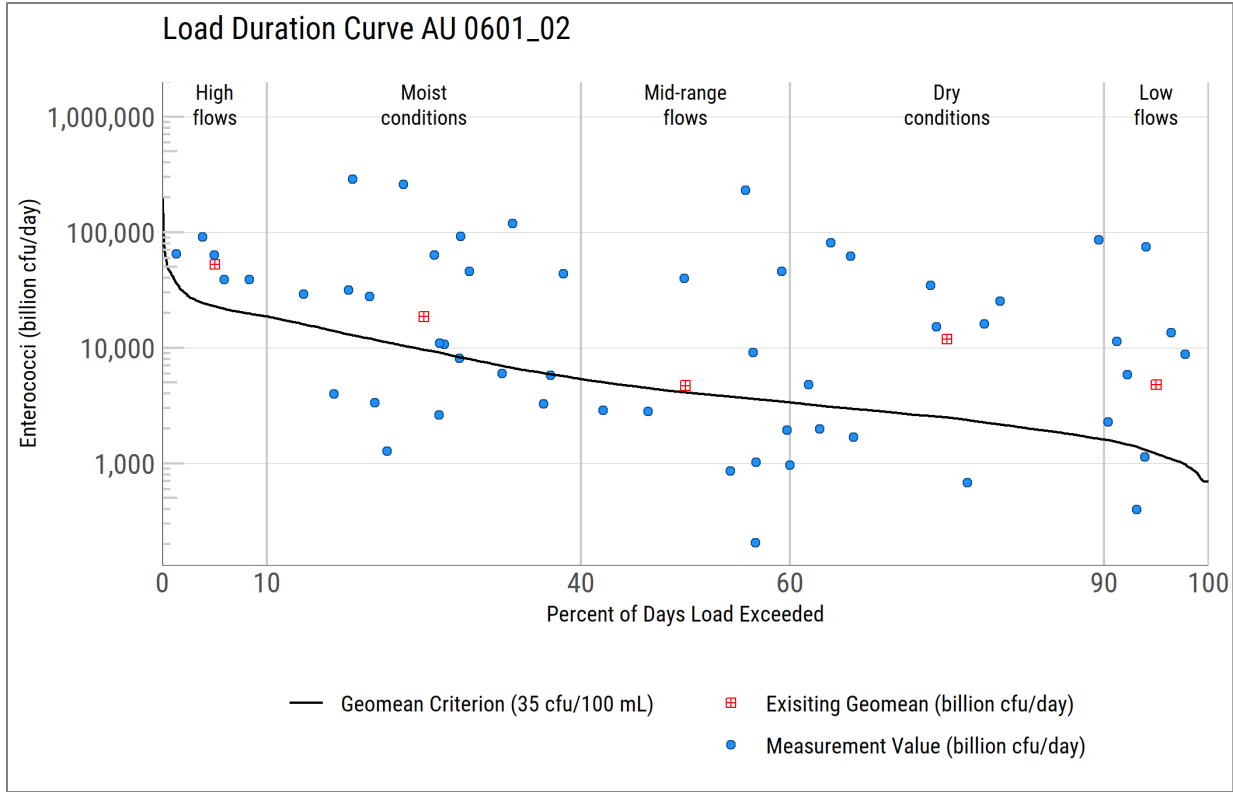
Figure 32. Load duration curve for Neches River Tidal (0601_02) at station 10566.
