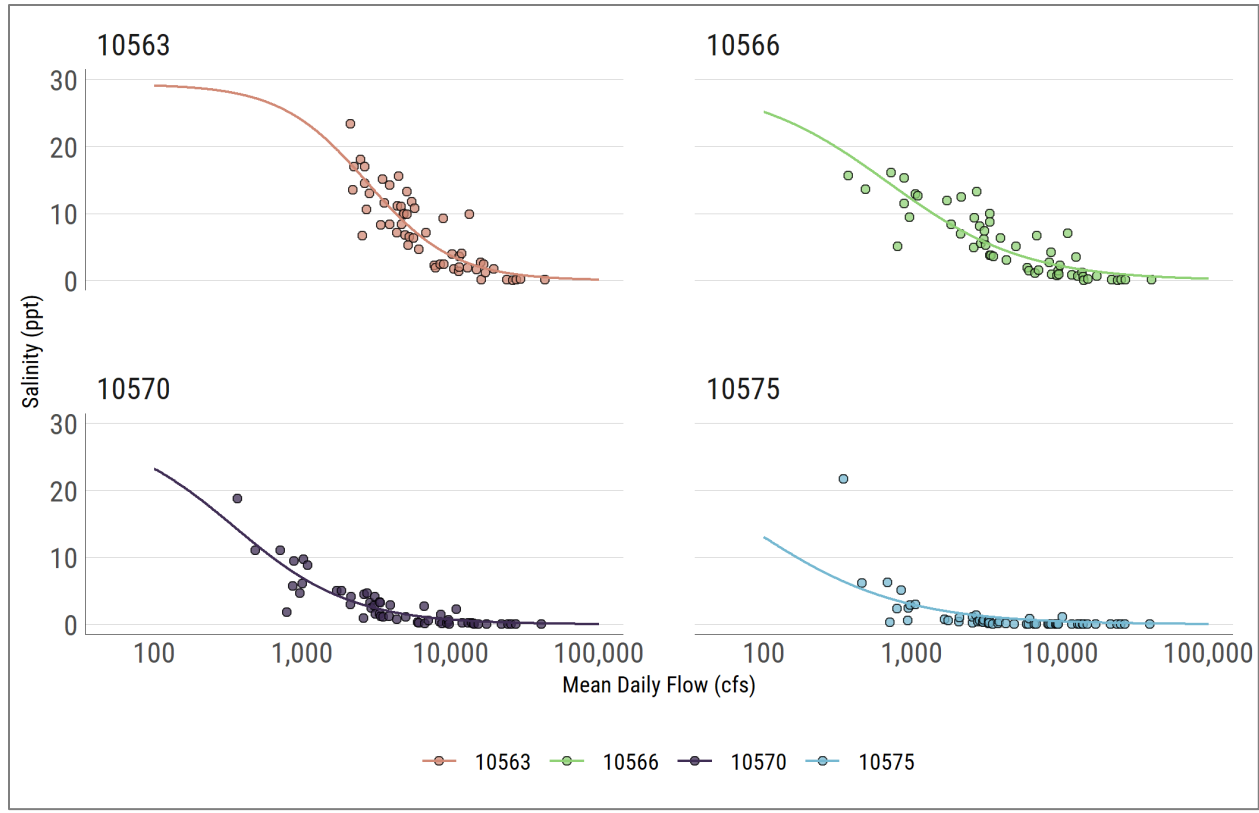
Figure A- 1. Salinity and streamflow regressions at each SWQM station.
