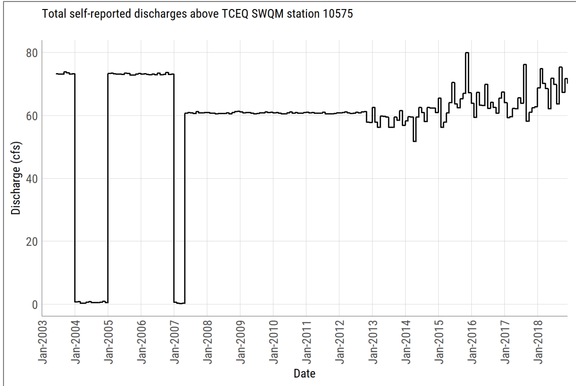
Figure 15. Reported discharge volumes for permitted facilities upstream of SWQM station 10575.
